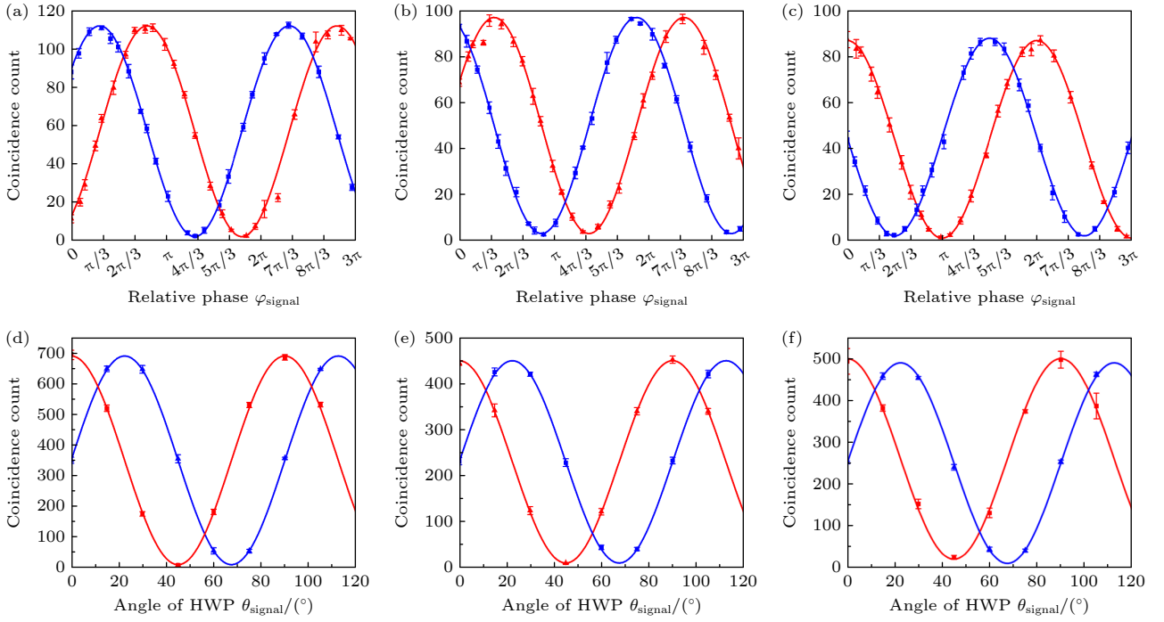
图2 time-bin 纠缠和偏振纠缠实验结果 (a) CH31&CH33 time-bin 纠缠双光子干涉条纹; (b) CH30&CH34 time-bin 纠缠双光子干涉条纹; (c) CH29&CH35 time-bin 纠缠双光子干涉条纹; (d) CH31&CH33 偏振纠缠双光子干涉条纹; (e) CH30&CH34 偏振纠缠双光子干涉条纹; (f) CH29&CH35 偏振纠缠双光子干涉条纹
